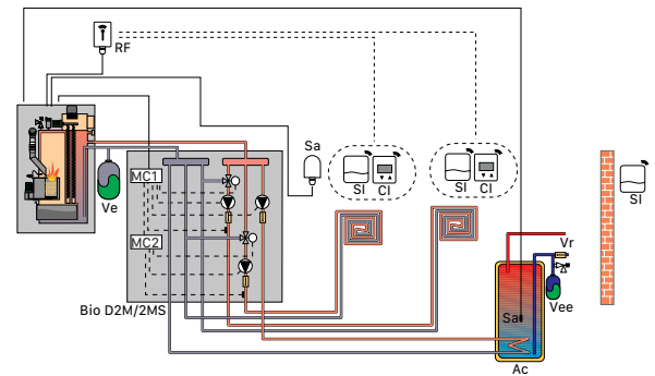
KIT BIO M + BT
