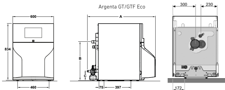
Argenta GTA/GTAF Eco
