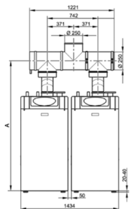
BK 250 (SGB 2x125 - 2x300)
