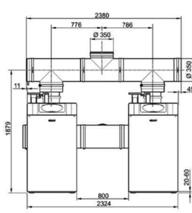
BK 350 (SGB 2x400 - 2x610)
